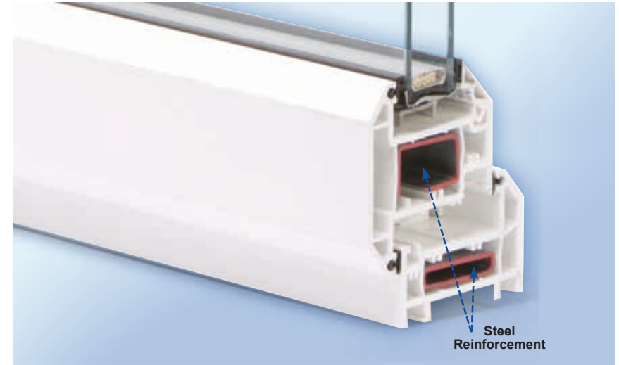
Diagram 1: Steel reinforcement
