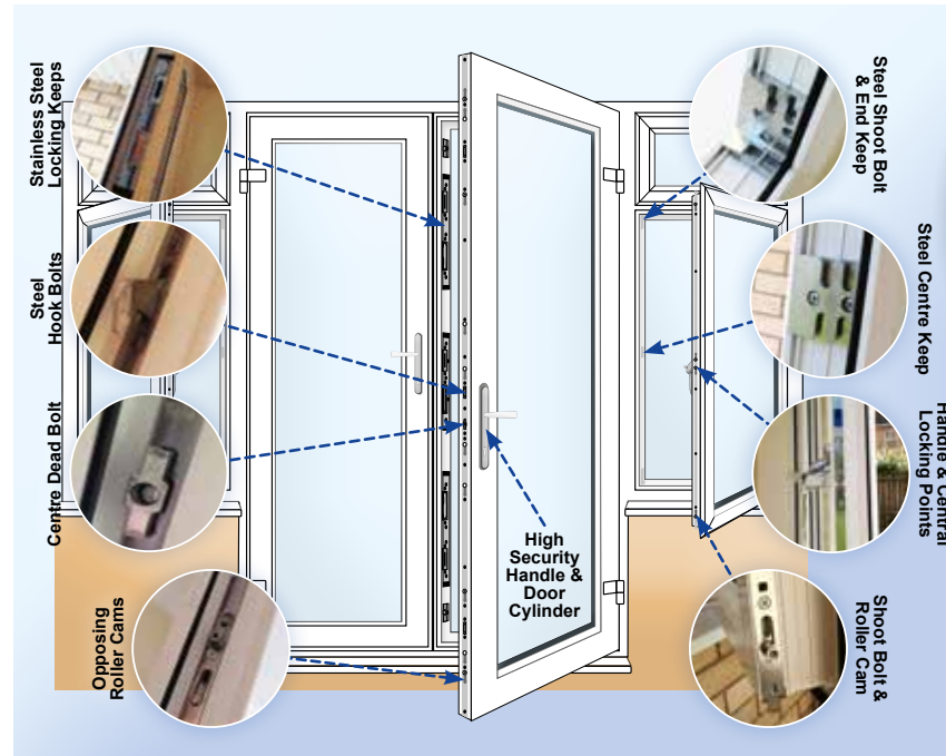
Diagram 2: Conservatory window and door security
